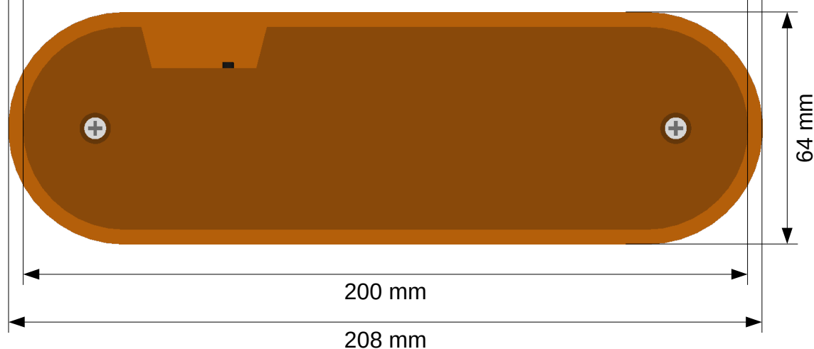
Bottom view
